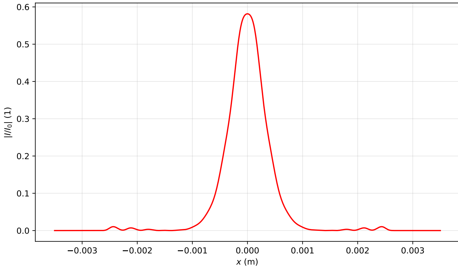
Intensity profile I(x, y = 0, z = 2.070)/I_0 , P_{in}=1.0P_{cr} , artificial time
